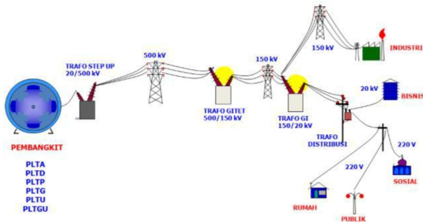
Figure 1. Schematic of electric power system
